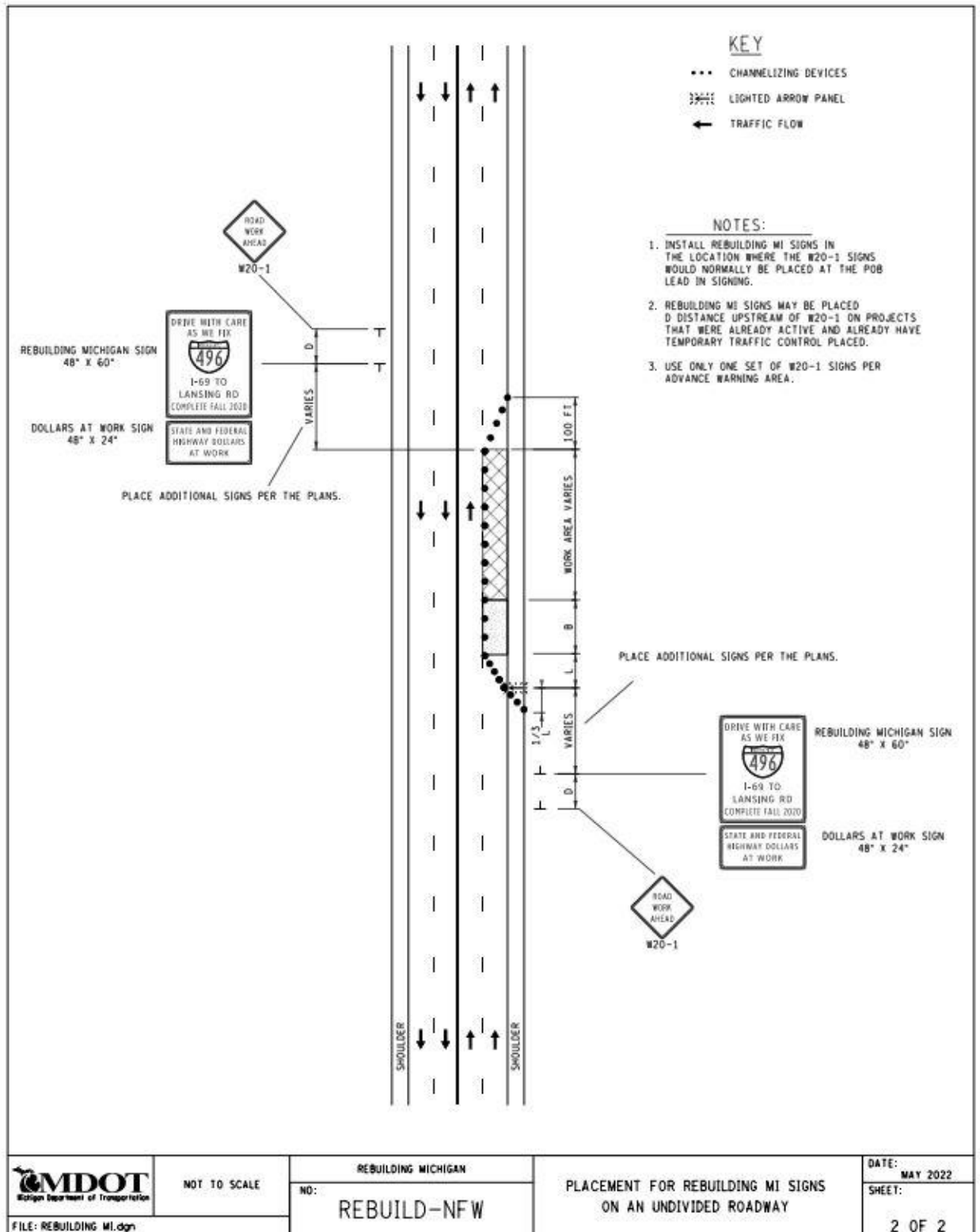
Figure 2: Detail for Placement for Rebuilding Michigan Signs and Plaques on Undivided Roadways
