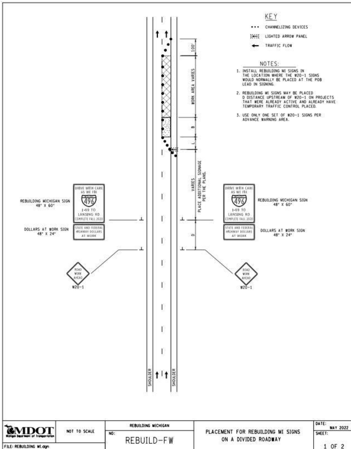
Figure 1: Detail for Placement for Rebuilding Michigan Signs and Plaques on Divided Roadways
