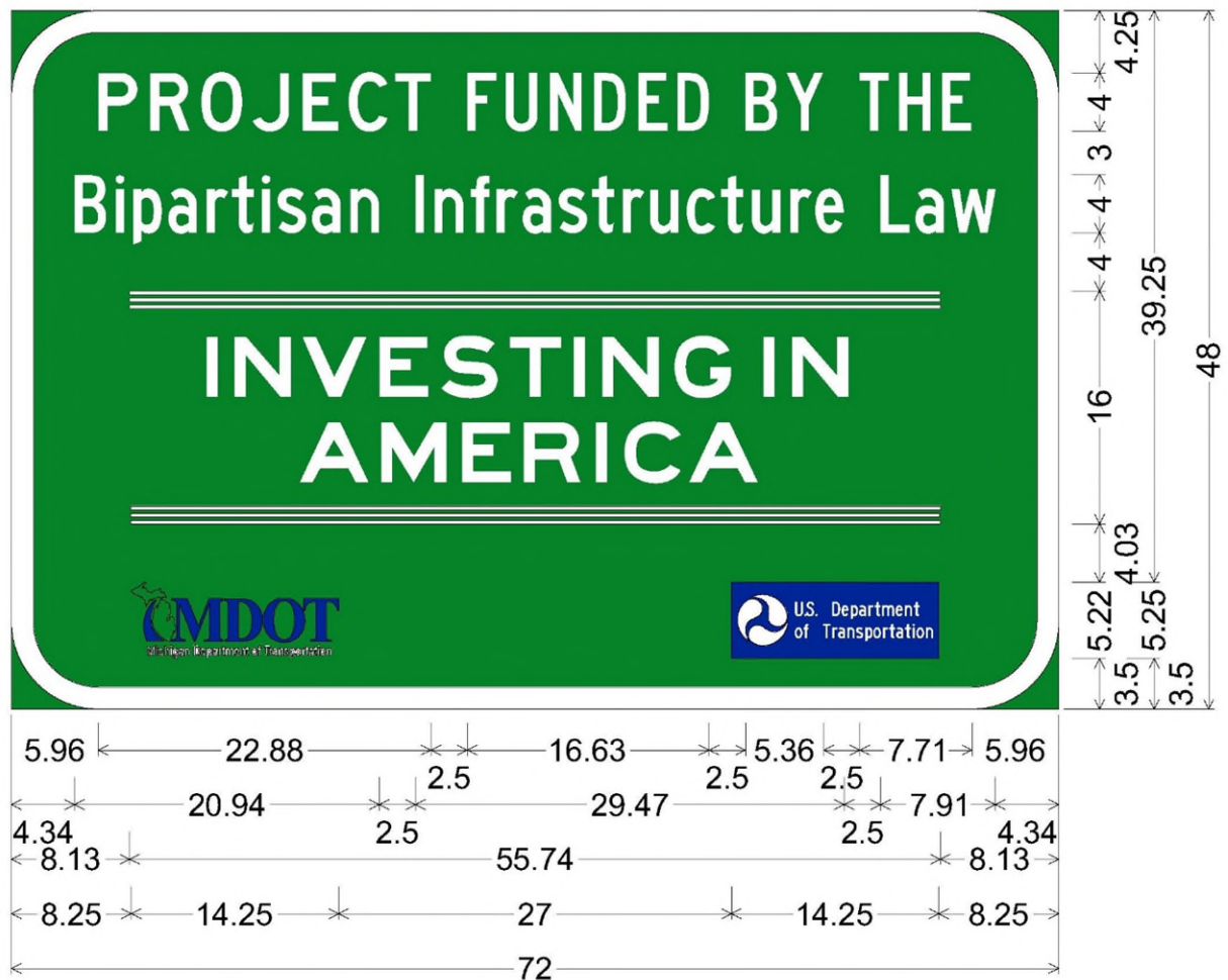
Detail 1: Bipartisan Infrastructure Law Sign for Non-Freeways
