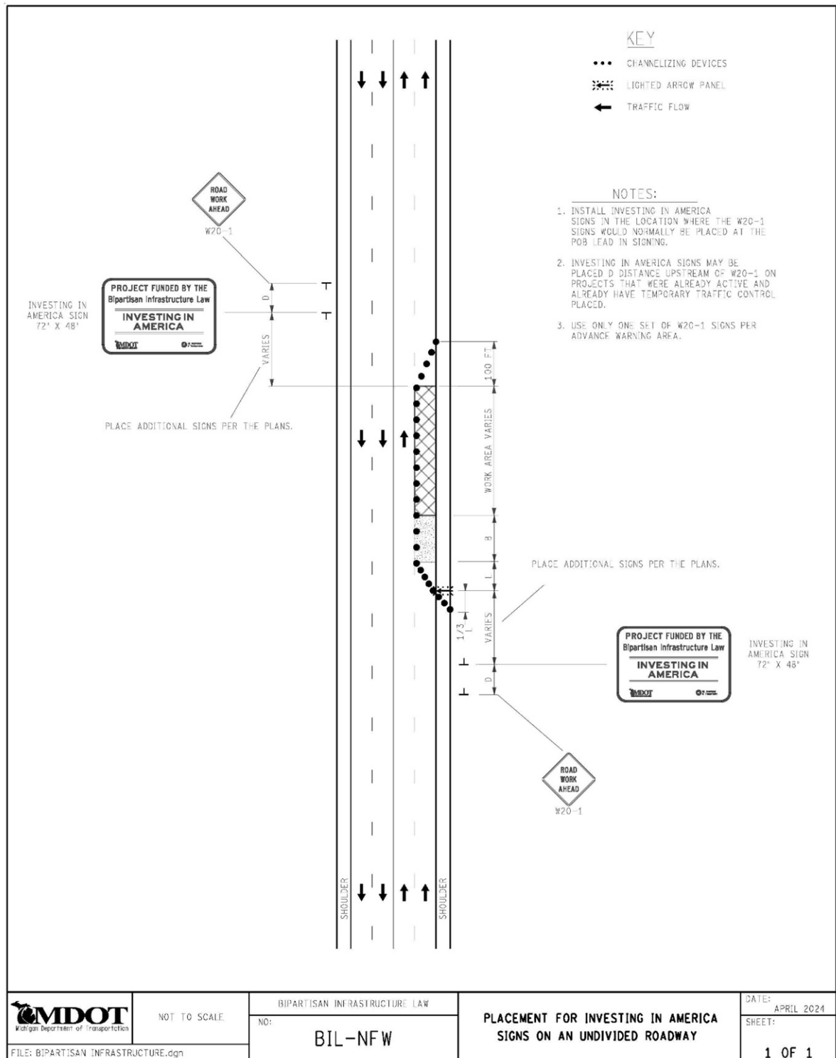
Figure 2: Detail for Placement for Bipartisan Infrastructure Law Signs on Undivided Non-Freeways
