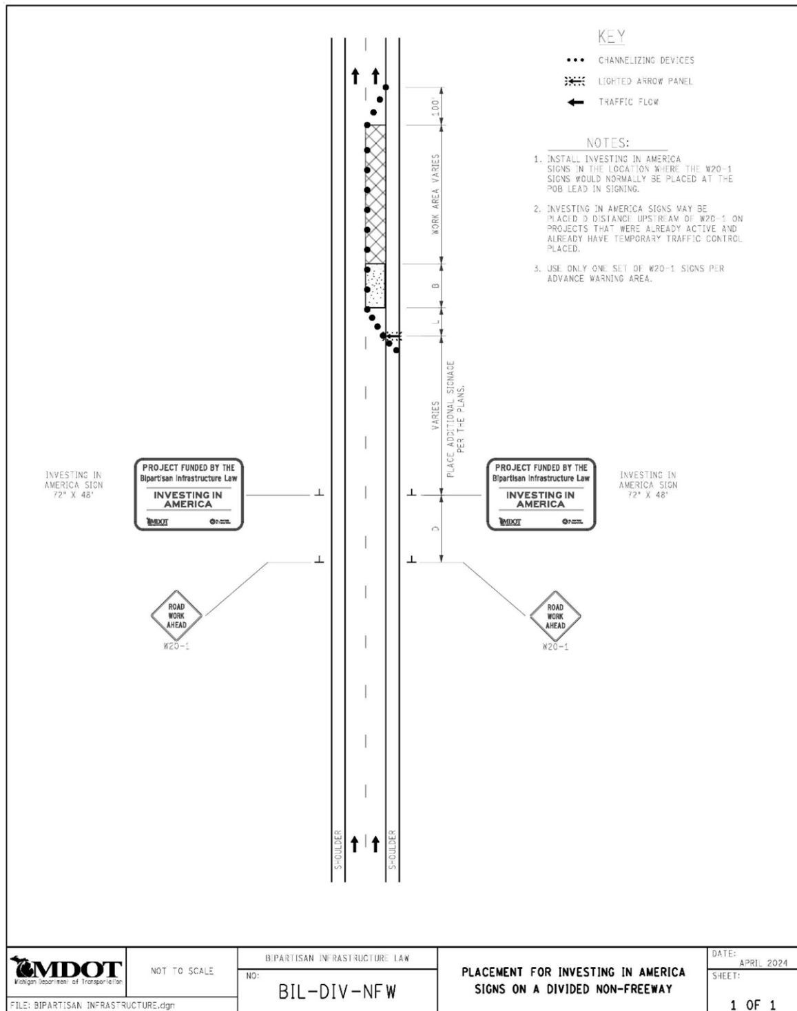
Figure 1: Detail for Placement for Bipartisan Infrastructure Law Signs on Divided Non-Freeways
