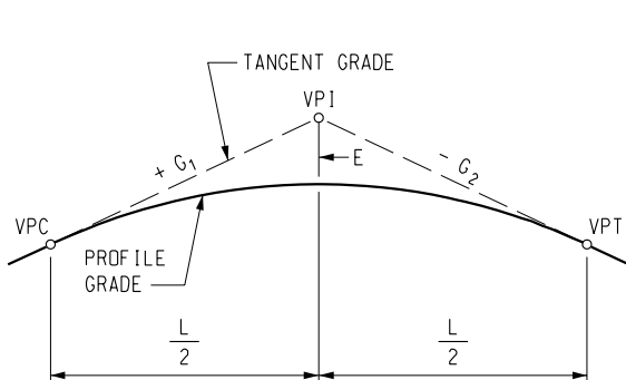
CREST VERTICAL CURVE
