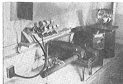
Figure 8. Spectrophotometric Assembly
