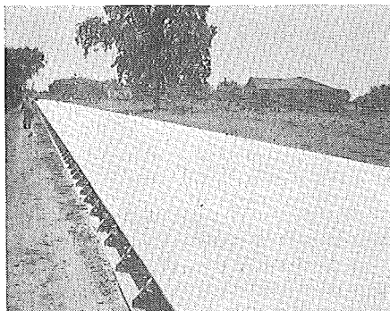
Figure 5. Uniform Coverage at the Rate of 204 sq. ft. per gal. with Pump Pressure of 200 p.s.i.
