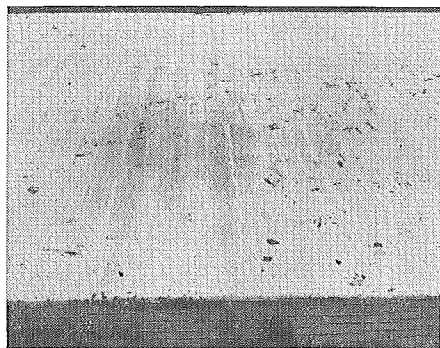
Figure 2. Ridging Effect Due to Clogging of Spray Nozzles—This picture was taken after removal of forms the following morning.
