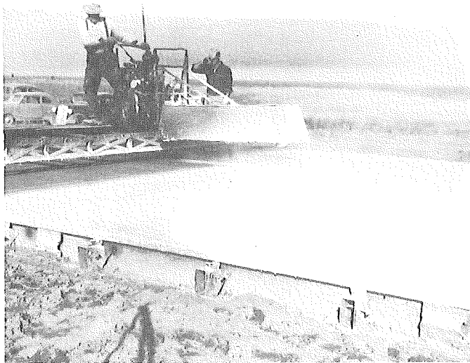
▲ FIGURE 1. DISTRIBUTOR USED IN EARLY FIELD TESTS. ENTIRE SPRAY UNIT IS BEING PULLED BY HAND ACROSS THE BRIDGE.
