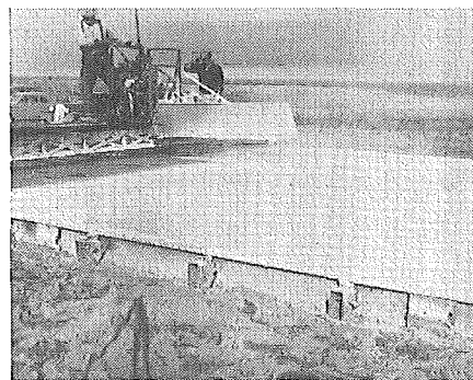
Figure 1. Distributor Used in Early Field Tests—Entire spray unit is being pulled by hand across the bridge.
