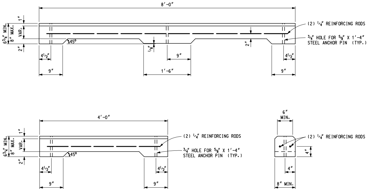
CONCRETE PARKING RAIL
