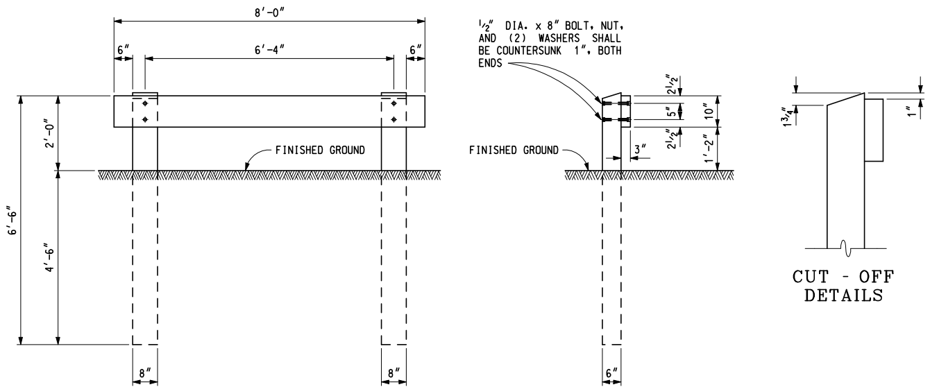
WOODEN BUMPER RAIL (FOR ANGLE PARKING)
