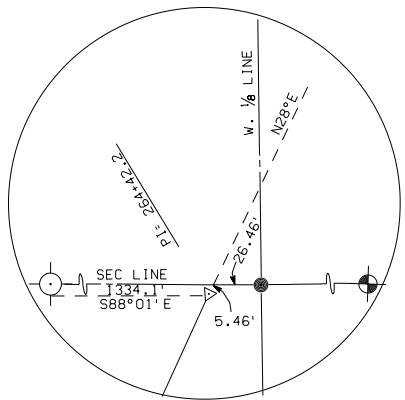
SKETCH SHOWING 1/8 COR TIE
